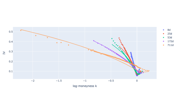
Figure 5.10: The deep smoother on real SPX quotes, 2018-01-08: market quotes with the fitted surface, on the day carrying the worst butterfly violation of the parametric benchmark. Source: Notebook 03.
