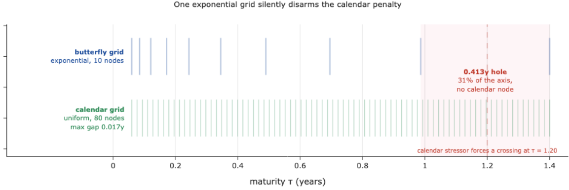
Figure 3.2: Constraint-specific collocation on the maturity axis [0.06, 1.4] of the synthetic stress experiments of Section 5.2. The literature’s exponential grid (top, ten nodes) crowds the short end, where the butterfly constraint bites, but leaves a 0.413-year gap at the long end, 31% of the axis with no calendar node (shaded). The calendar stressor of Section 5.2 forces its crossing inside that gap (dashed), so the penalty reads zero on a surface that is violating. Giving the calendar constraint its own uniform grid (bottom, 80 nodes) brings the maximal gap down to 0.017 years.
