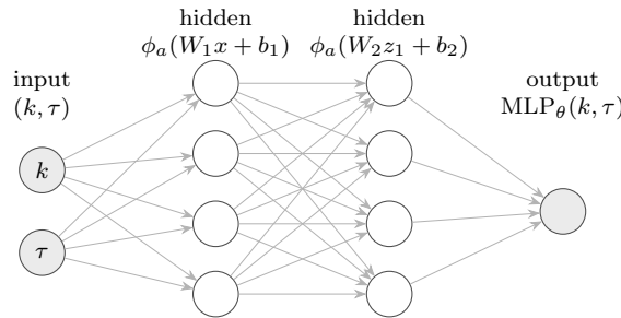
Figure 3.4: A multilayer perceptron (3.3): it maps one point of the surface to one number . Each arrow is a learned weight; each circle applies the activation \phi_a . To obtain a whole surface, the network is evaluated point by point, and the parameters \theta are fitted to one day’s quotes.
